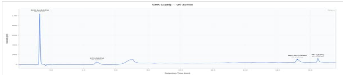
KLOW 80mg 80mg - AS-KLOW80-2: UV Chromatogram
